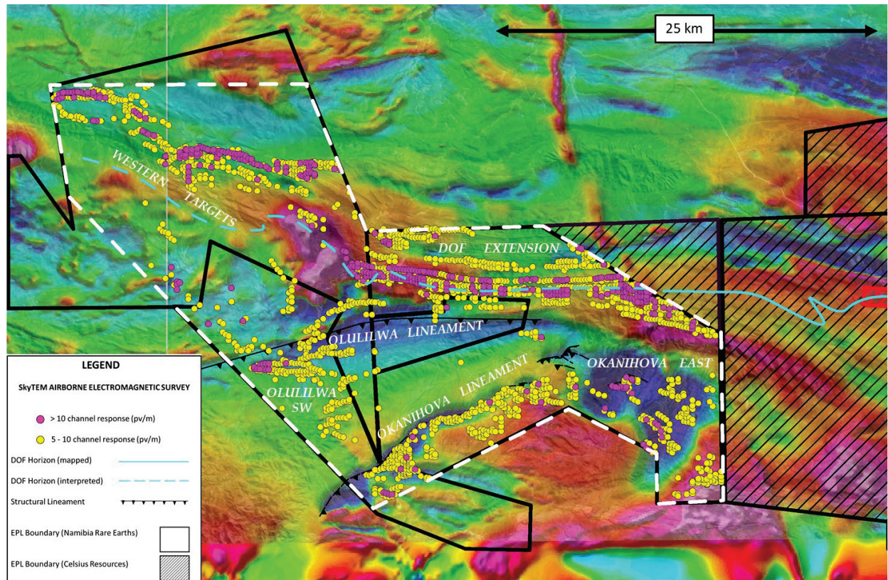
Figure 6 – Kunene Co-Cu Project Area showing SkyTEM airborne survey area (white dash) and preliminary EM conductor picks for 5-10 channel and > 10 channels responses. Responses for < 5 channels not shown. Channel responses are provided in picovolts/meter. Background image is total magnetic intensity from the Namibian Geological Survey database combined with satellite surface topography.
