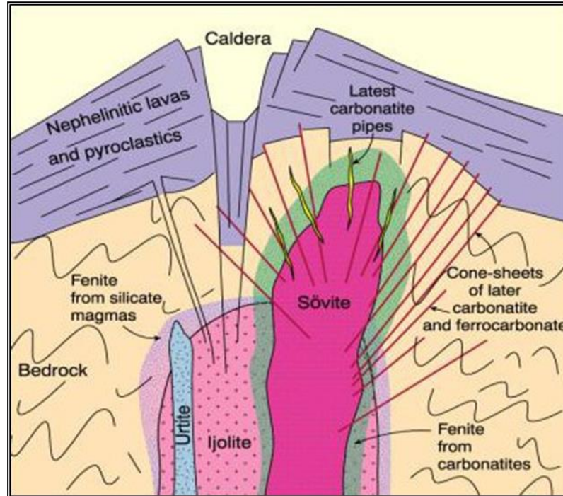
Figure 8-1 General cross-sectional model for an alkali silicate-carbonate intrusive complex (after Le Bas, 1987)
