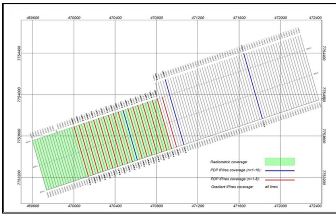
Figure 9-6 Area 4 grid showing ground geophysical coverage
