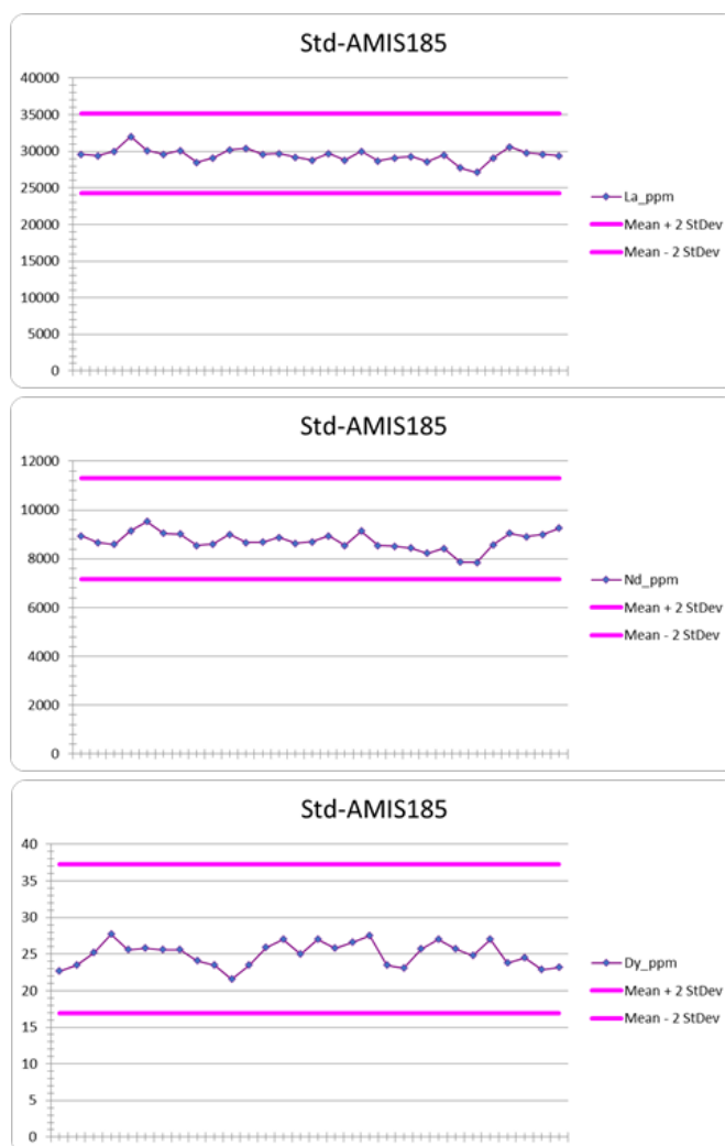
Figure 11-8 Analyses of the CRM AMIS0185 for selected REE in Area 2B
