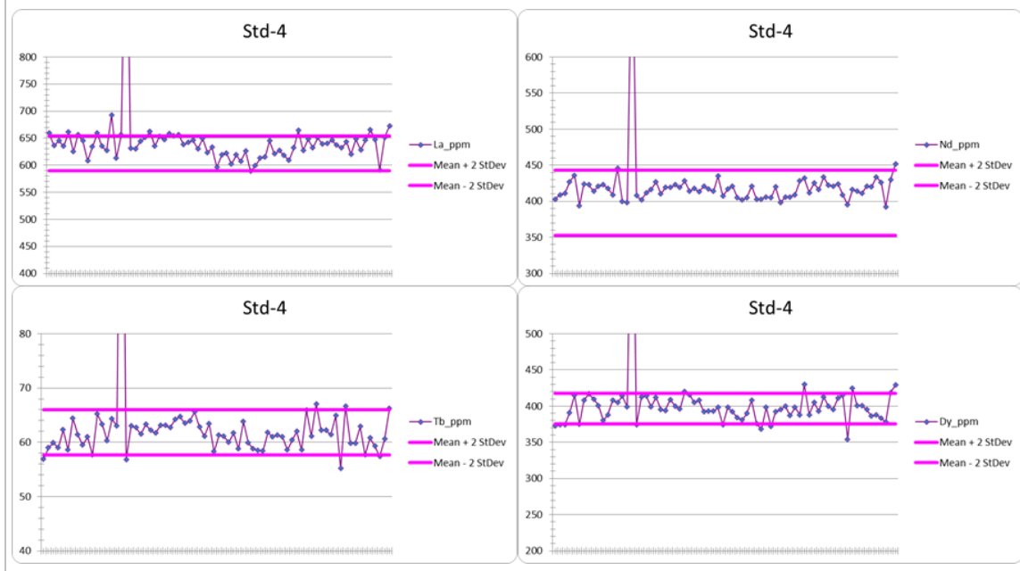
Figure 11-11 Analyses of the Standard STD4 for selected REE in Area 4
