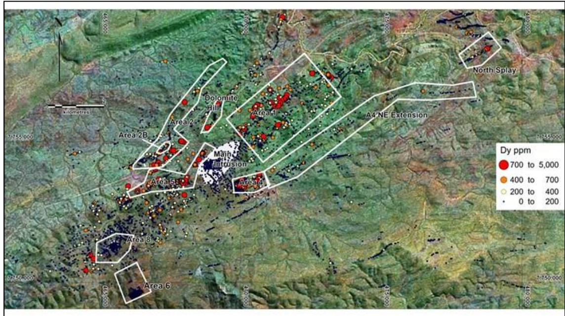
Figure 9-2 Priority exploration areas defined by Dy in surface lithogeochemistry samples
