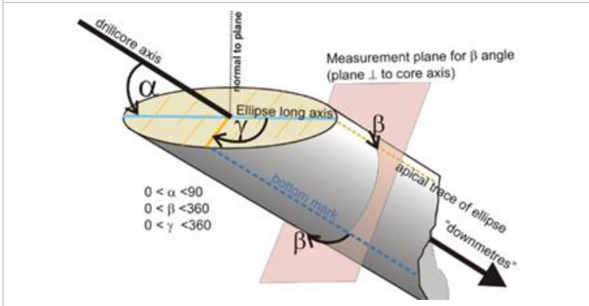
Figure 11-1 Illustration of the alpha, beta, and gamma angles in core
