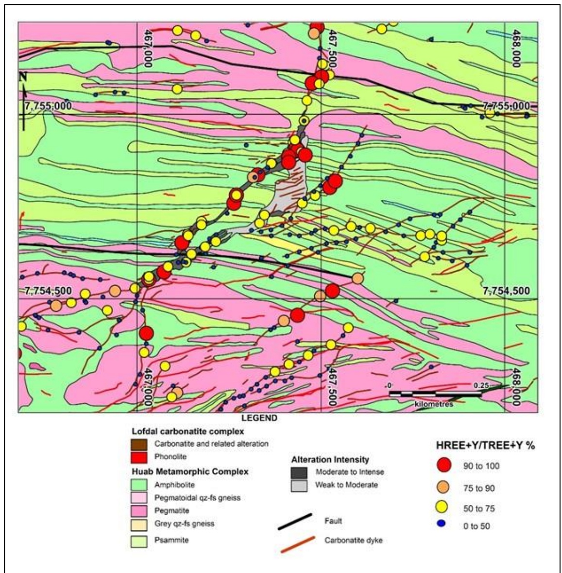
Figure 7-17 (HREE+Y)/(TREE+Y) % in surface grab samples in Area 2
