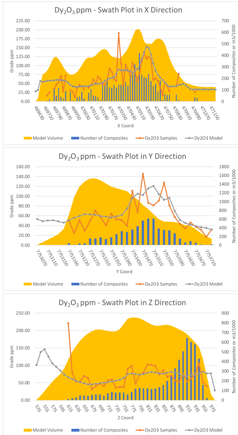
Figure 14-9 Swath Plot Validation for Dy 2 O 3
