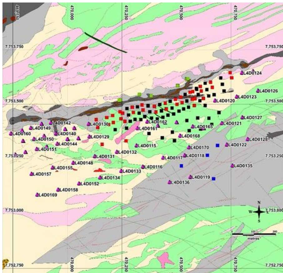
Figure 10-3 Plan showing drillhole collars in Area 4
