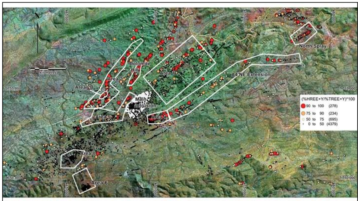
Figure 9-3 Priority exploration areas defined by HREE/TREE ratio in surface lithogeochemistry samples
