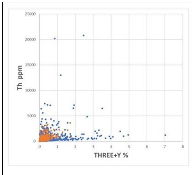
Figure 7-26 THREE versus Th in trench and drillhole core samples
